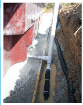
Geo-Hydro Valve™
